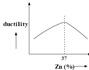
Variation of ductility of brass with percentage of zinc.
