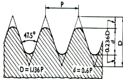
British Association thread
