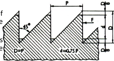
Buttress thread Theoretical depth D = P Actual depth d = \frac{3}{4} D
